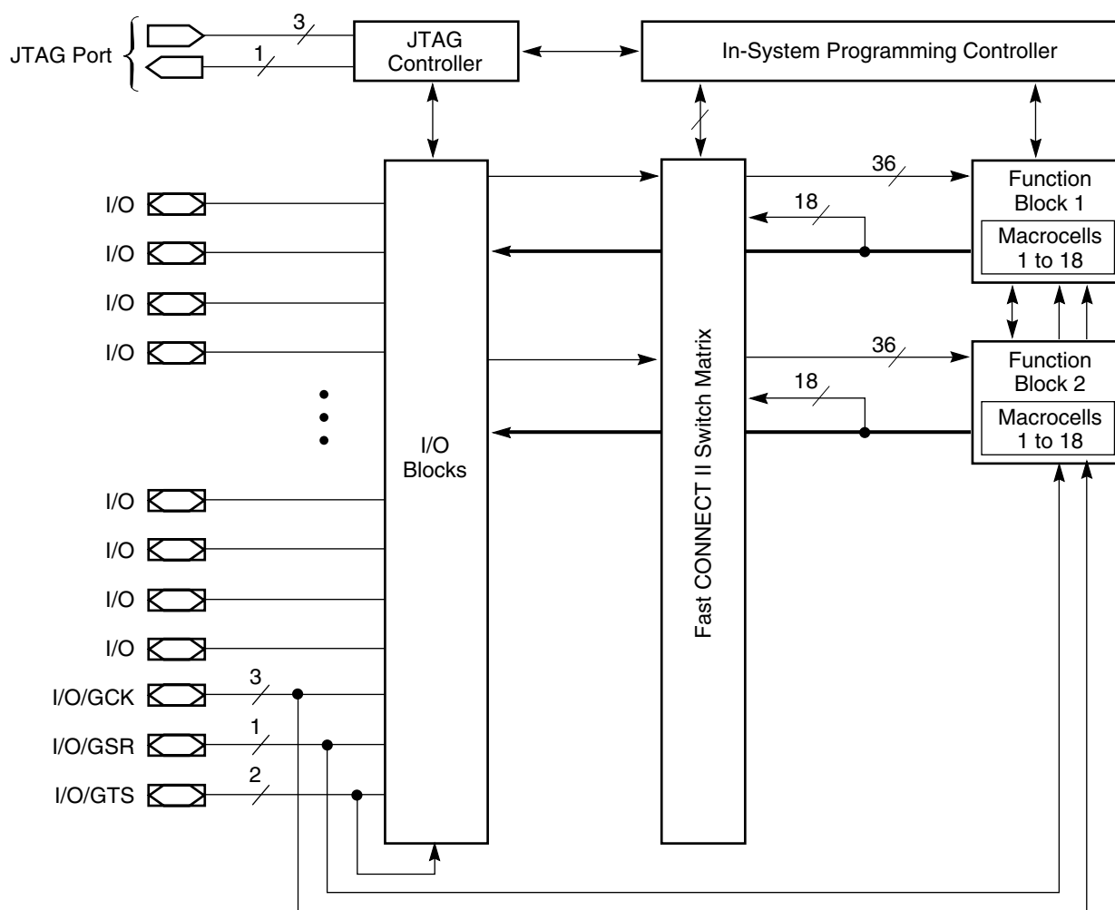
Figure 2: XC9536 Architecture
