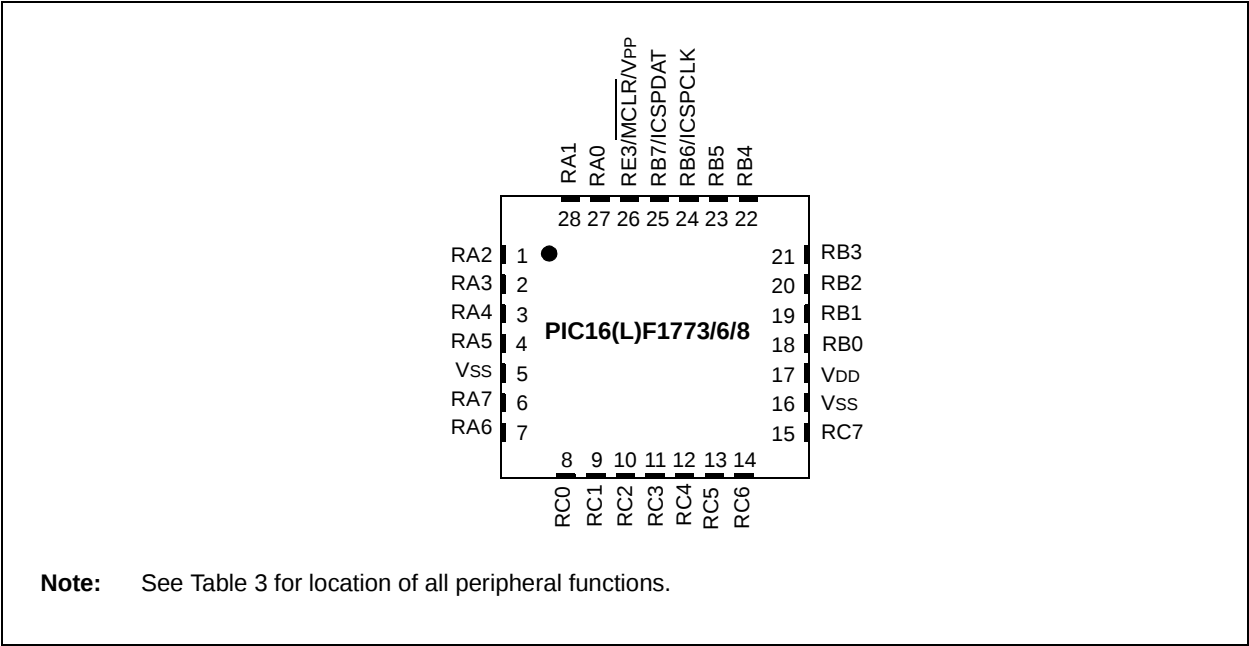
FIGURE 2: 28-PIN UQFN (6x6x0.5 mm)
