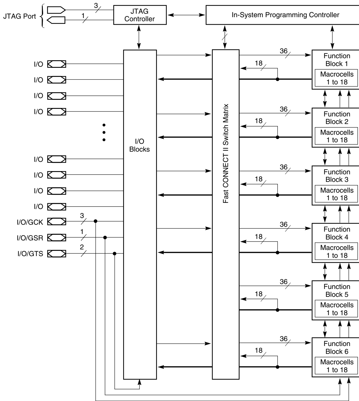
Figure 2: XC95108 Architecture
