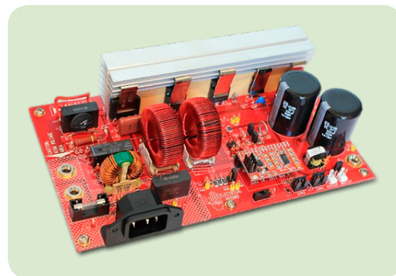
ADP1048 600 W interleaved evaluation board.
