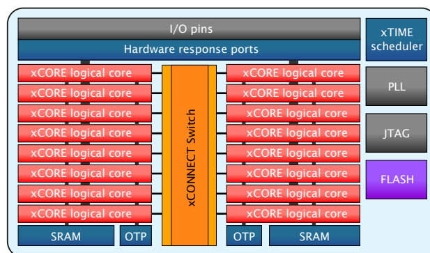
xCORE-200™ XLF216
