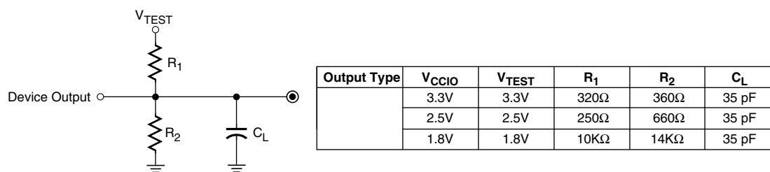
Figure 3: AC Load Circuit
