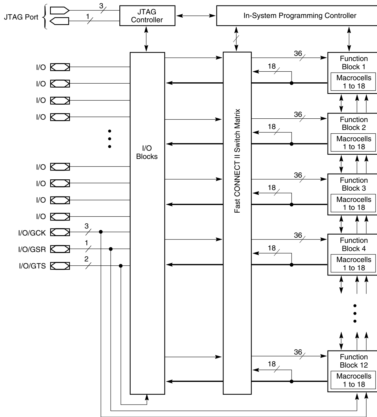
Figure 2: XC95216 Architecture
