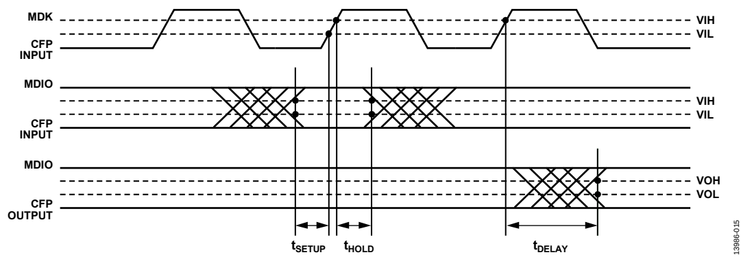
Figure 7. MDIO Timing
