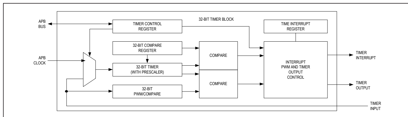
Figure 7. 32-Bit Timer
