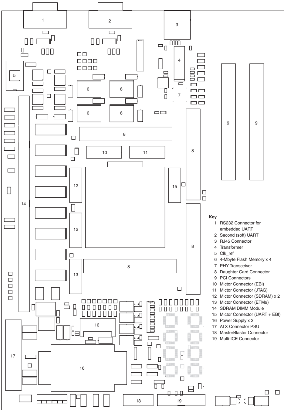
Figure 6. Excalibur Development Board
