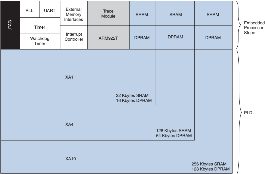
Figure 1. Excalibur Architecture
