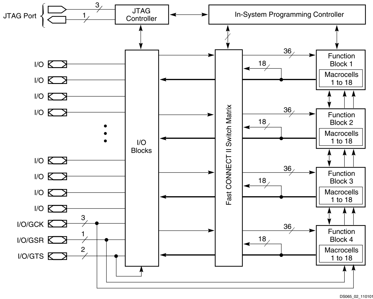
Figure 2: XC9572 Architecture
