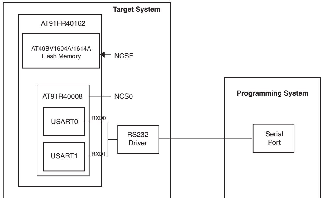
Figure 7-1. Flash Uploader
