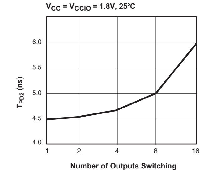
DS095_02_053103 Figure 2: Derating Curve for T PD
