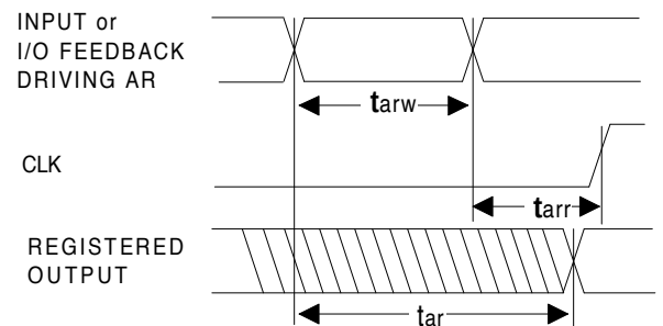
Asynchronous Reset
