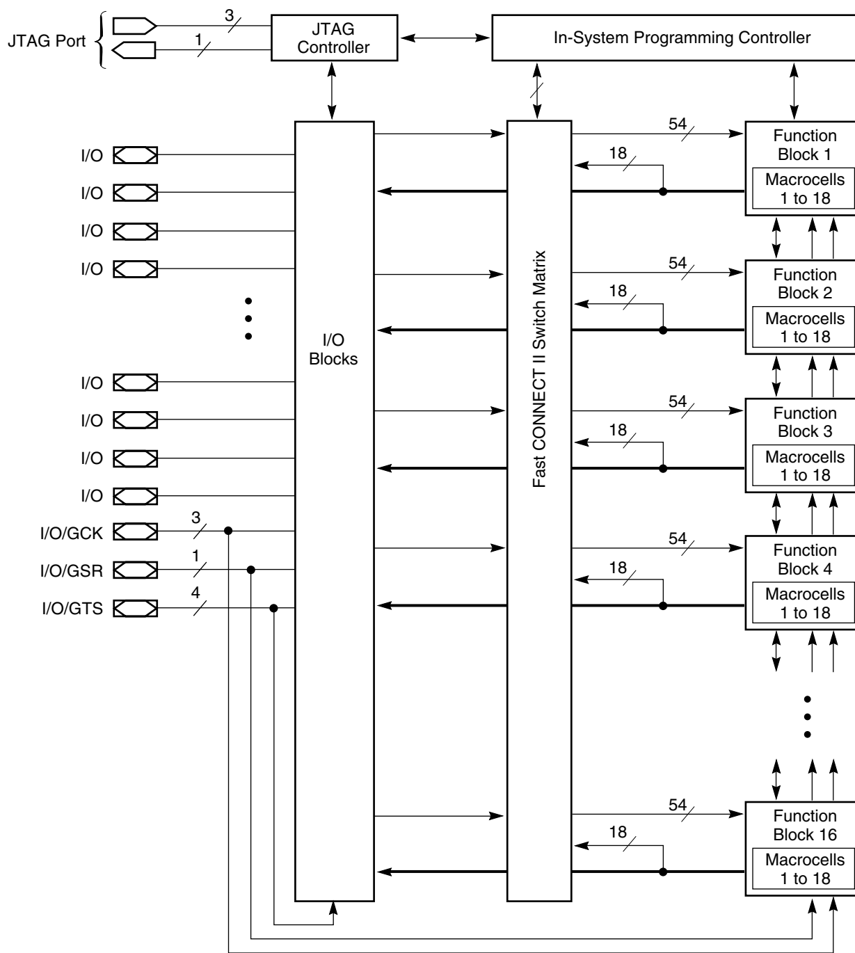
Figure 2: XC95288XL Architecture
