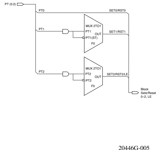
Figure 5. Set/Reset Generator
