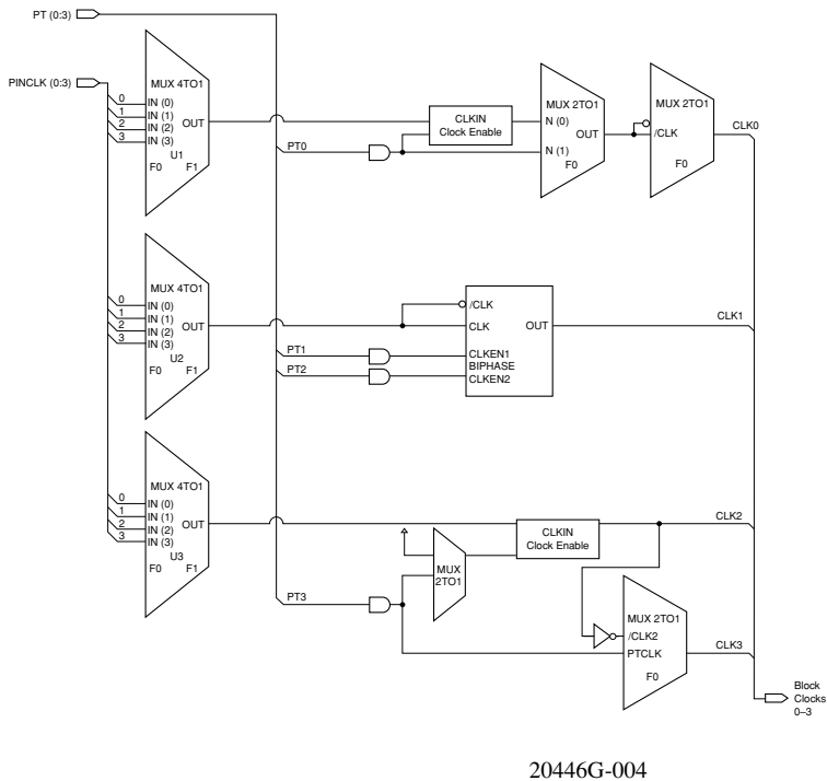
Figure 4. Clock Generator
