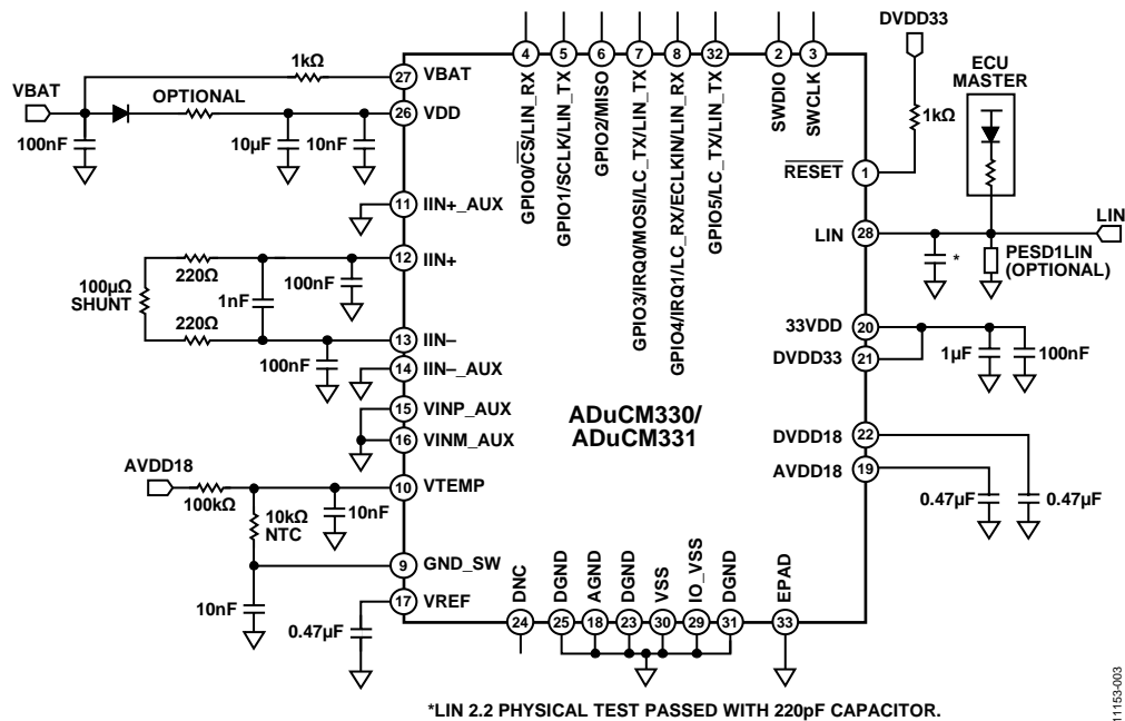
Figure 3. Recommended Schematic
