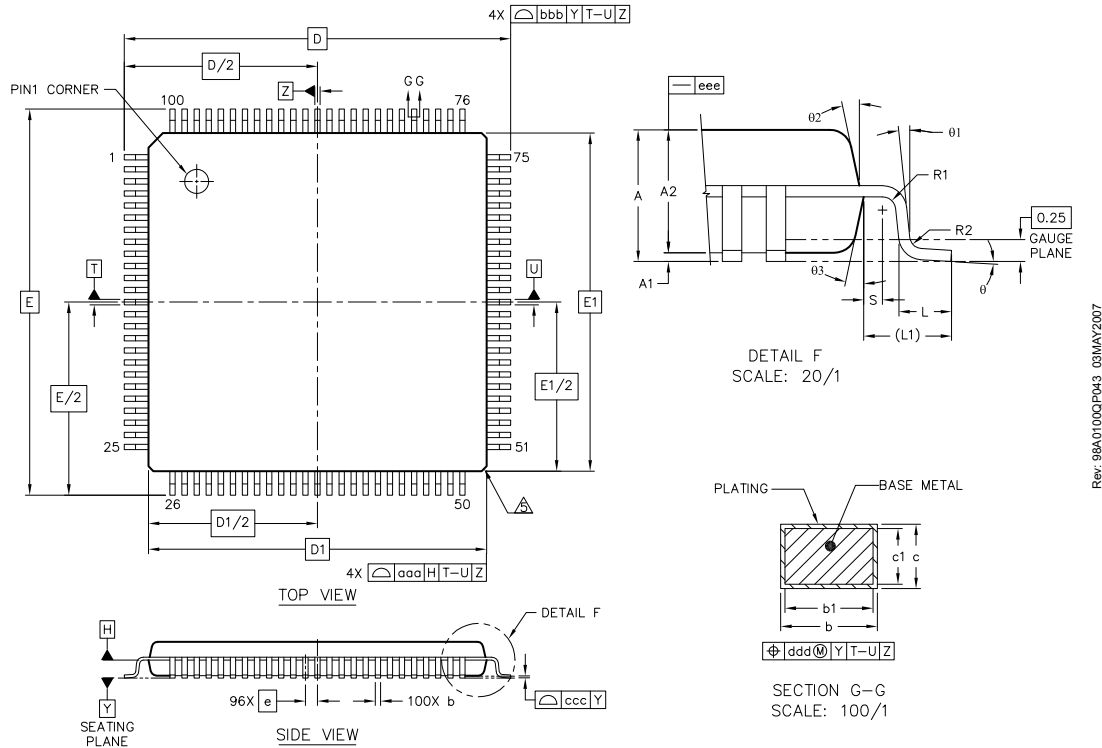
Figure 7.1. LQFP100
