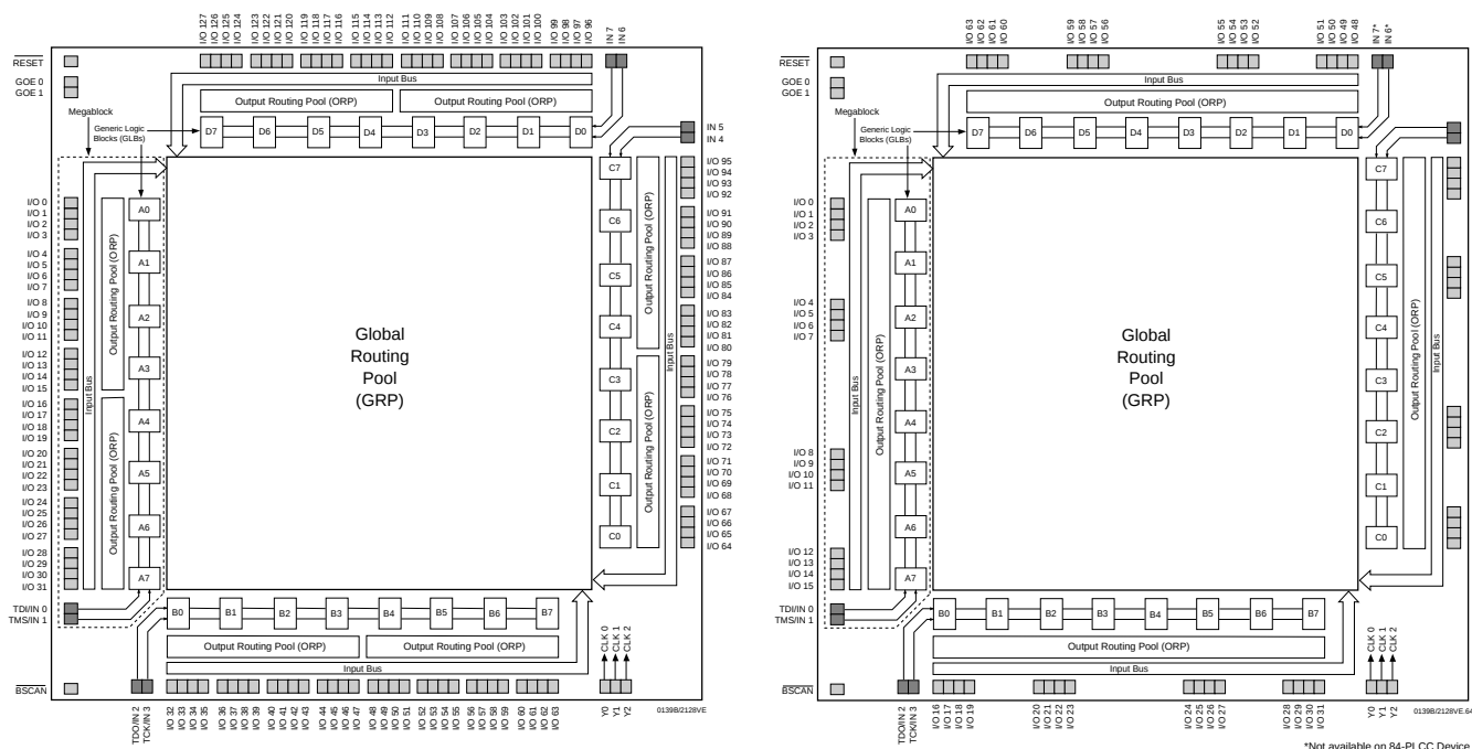
Figure 1. ispLSI 2128VE Functional Block Diagram (128-I/O and 64-I/O Versions)
