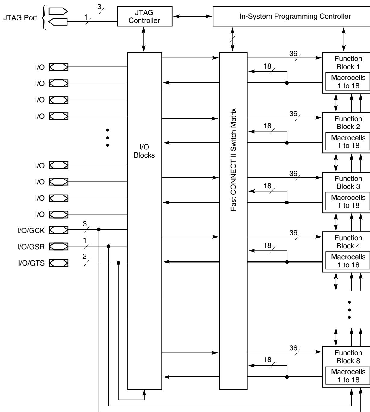
Figure 2: XC95144 Architecture
