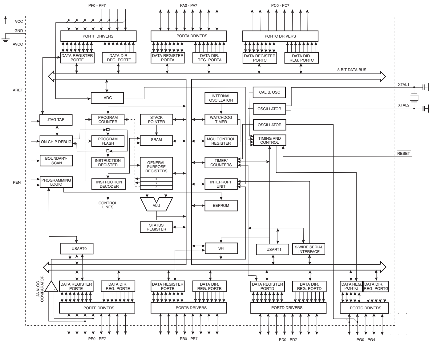
Figure 2. Block Diagram
