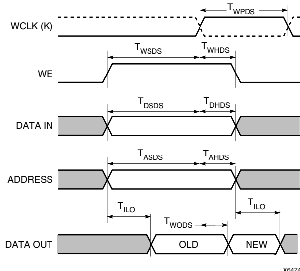
Dual-Port RAM
