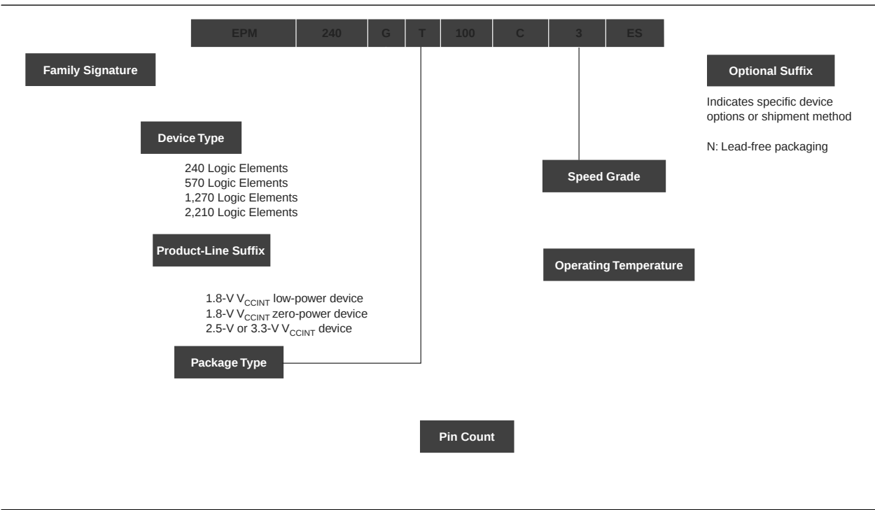
Figure 6–1. MAX II Device Packaging Ordering Information
