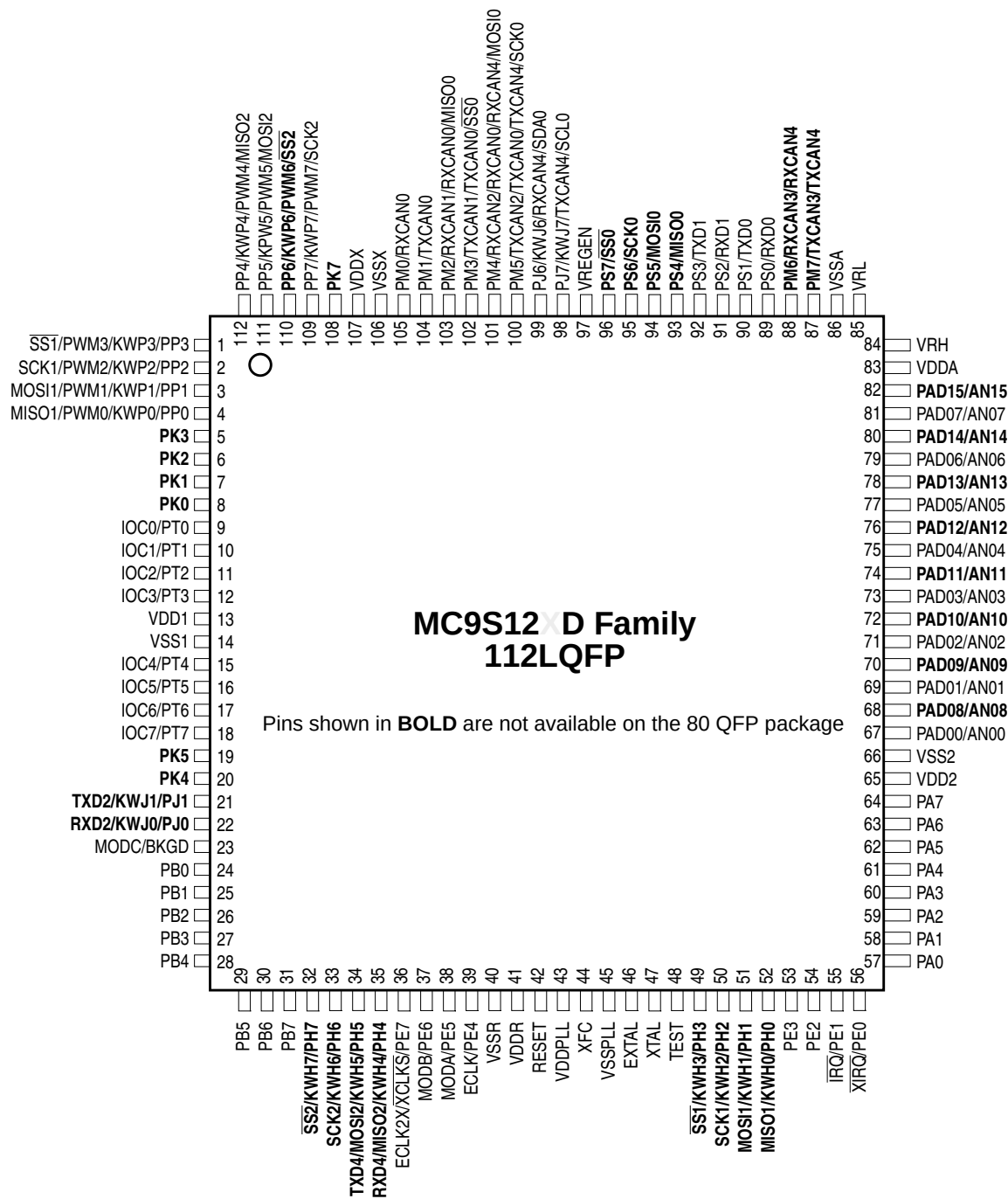
Figure 2. MC9S12 D Family Pin Assignments for 112-pin LQFP Package
