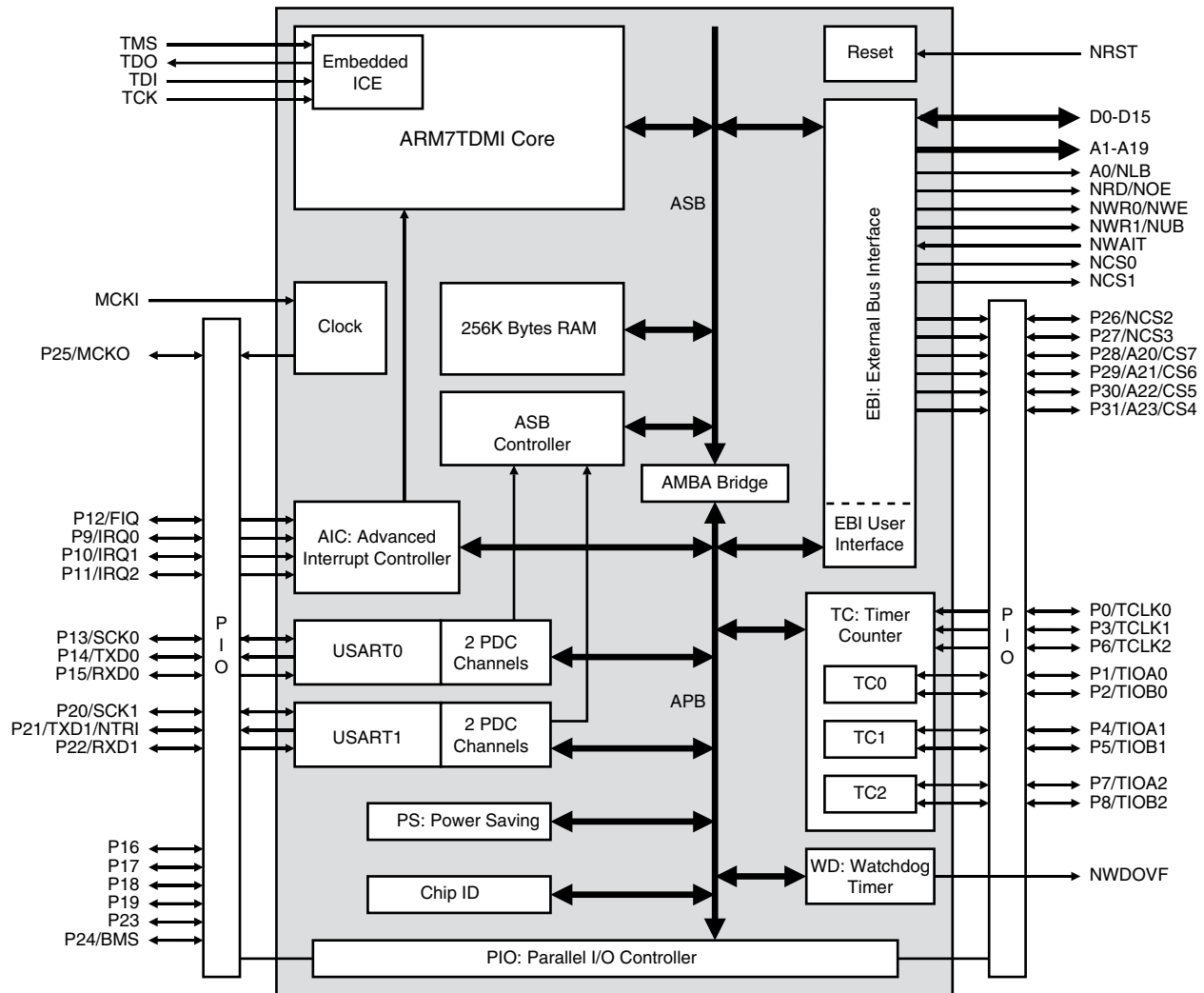
Figure 4-1. AT91R40008
