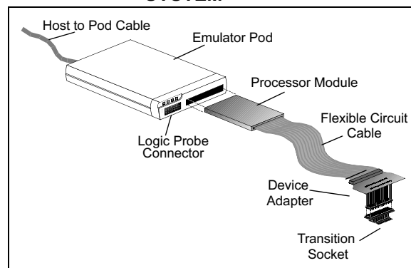
FIGURE 2-1: MPLAB ICE 2000 EMULATOR SYSTEM
