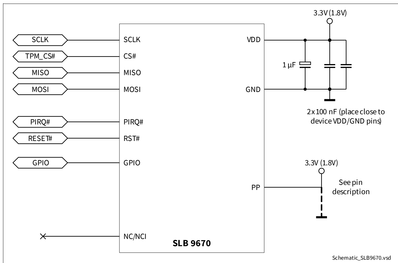
Figure 3-2 Typical Schematic
