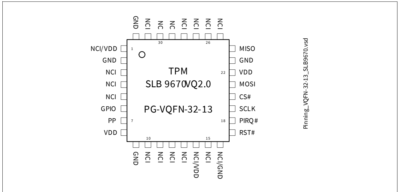
Figure 3-1 Pinout of the SLB 9670VQ2.0 (PG-VQFN-32-13 Package, Top View)
