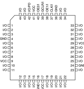
TQFP Top View
