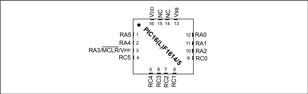
FIGURE 5: 16-PIN QFN
