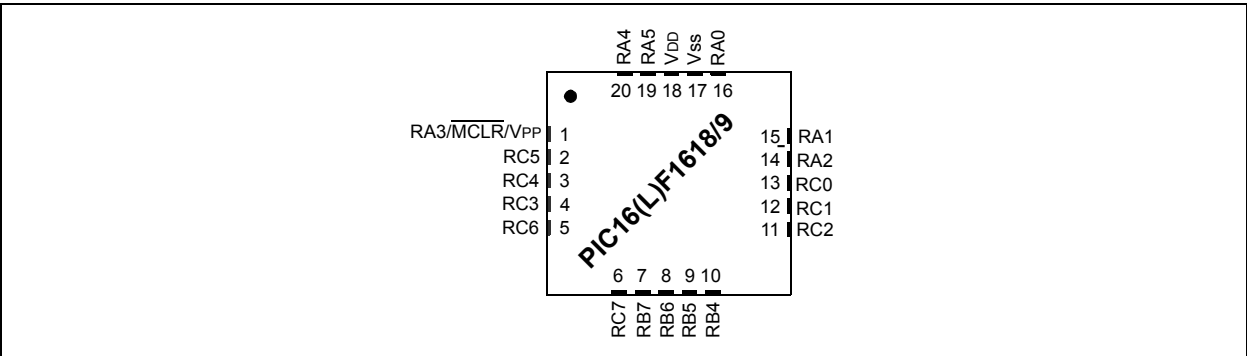
FIGURE 7: 20-PIN QFN
