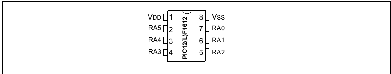
FIGURE 1: 8-PIN PDIP, SOIC, DFN, UDFN
