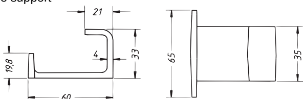
Cable support
