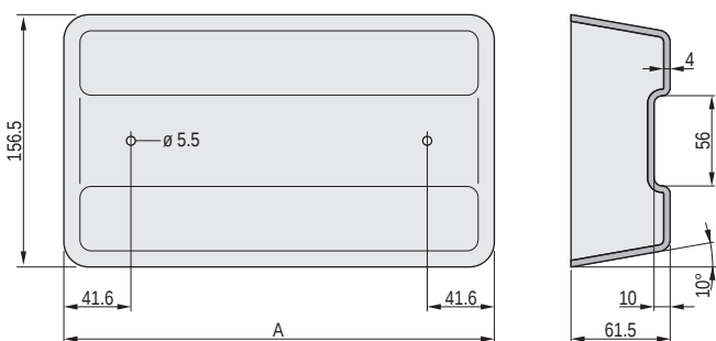
Cable support
