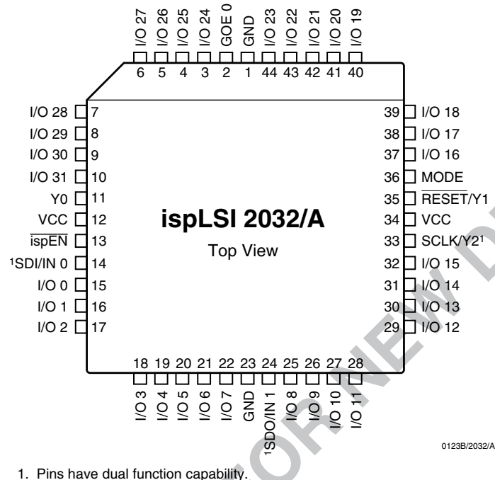
ispLSI 2032/A 44-Pin PLCC Pinout Diagram
