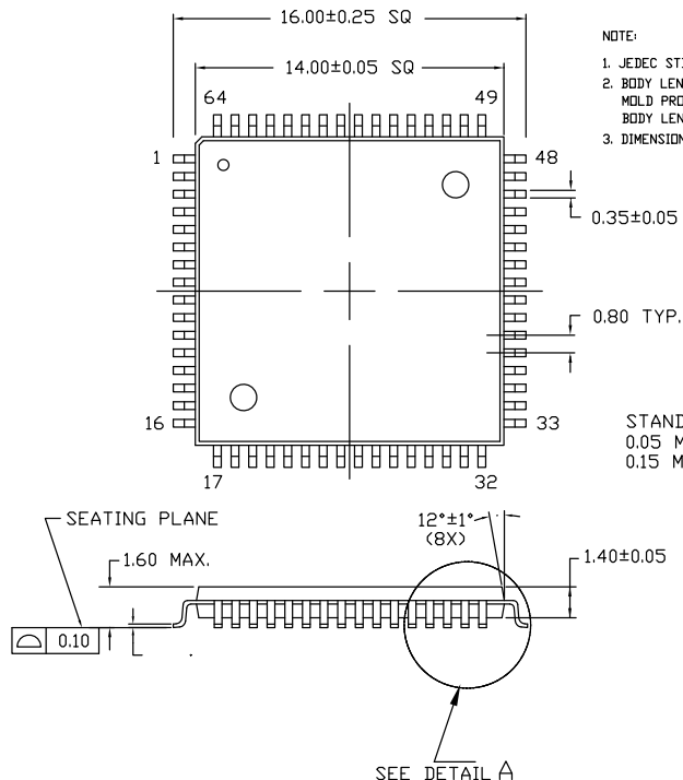
Figure 12. 64-pin TQFP (14 × 14 × 1.4 mm) Package Outline, 51-85046
