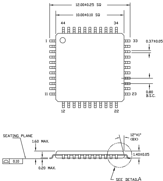
Figure 11. 44-pin TQFP (10 × 10 × 1.4 mm) Package Outline, 51-85064
