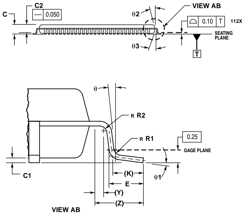
Figure 6. 112-pin LQFP Mechanical Dimensions (case no. 987)
