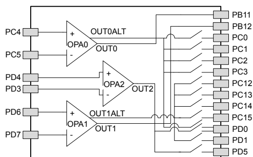
Figure 5.8. Opamp Pinout
