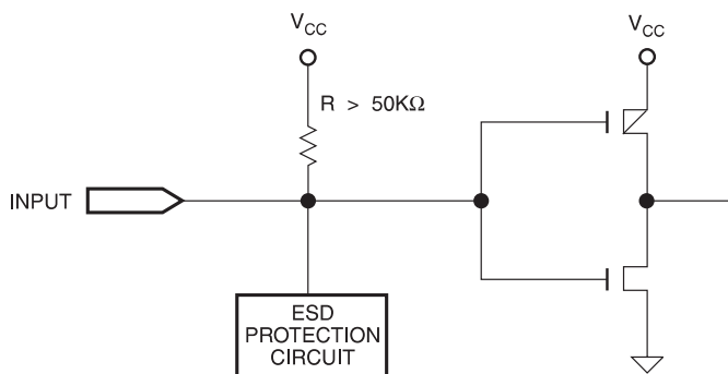
Figure 14-1. Input Diagram
