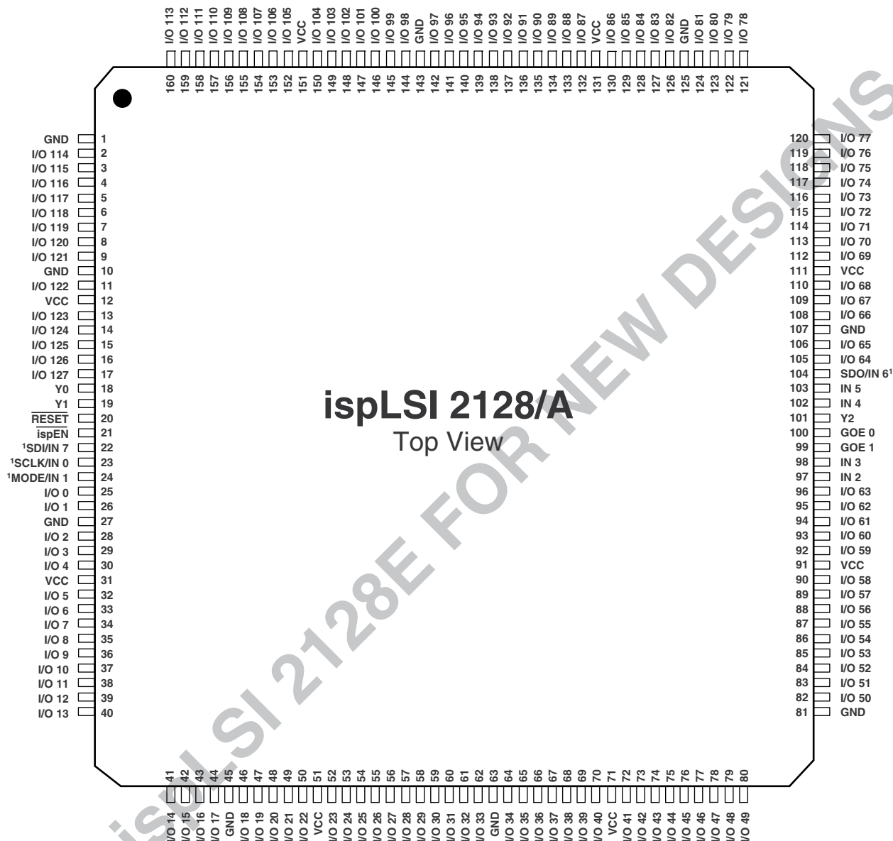
ispLSI 2128/A 160-Pin PQFP Pinout Diagram
