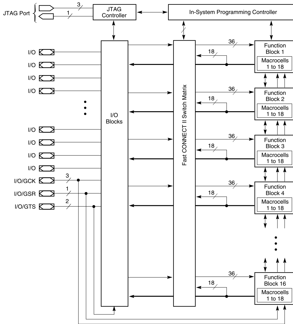
Figure 2: XC95288 Architecture
