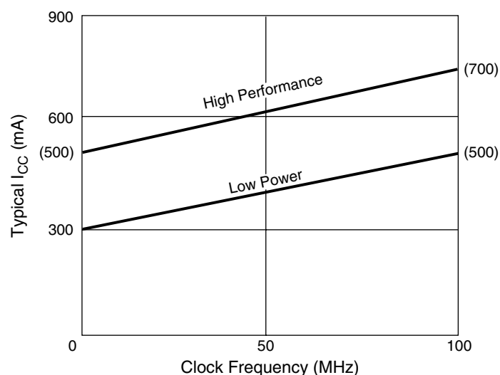
Figure 1: Typical I_{CC} vs. Frequency for XC95288
