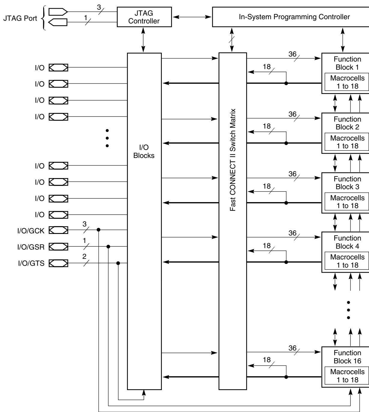
Figure 2: XC95288 Architecture
