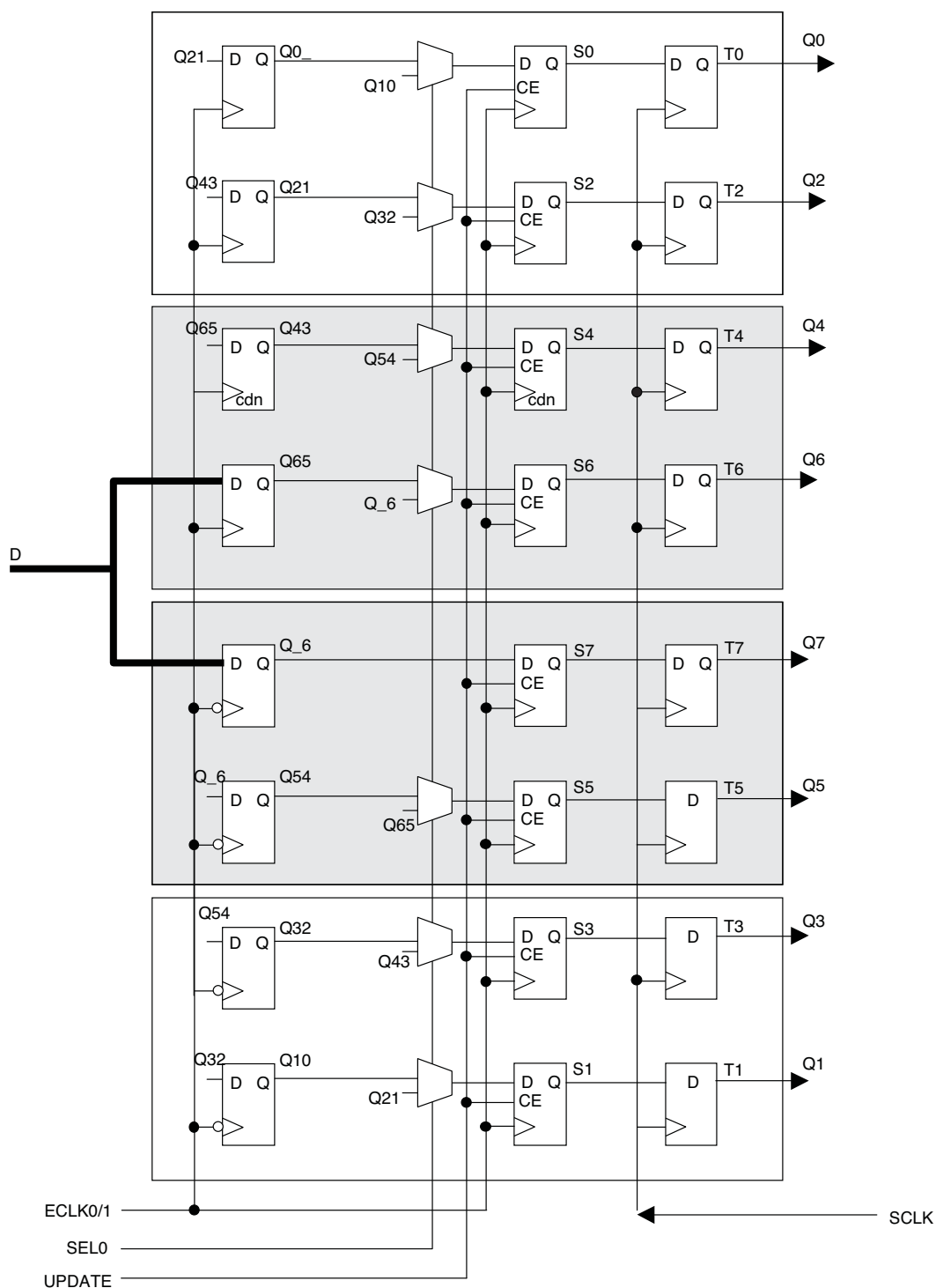
Figure 2-13. Input Gearbox
